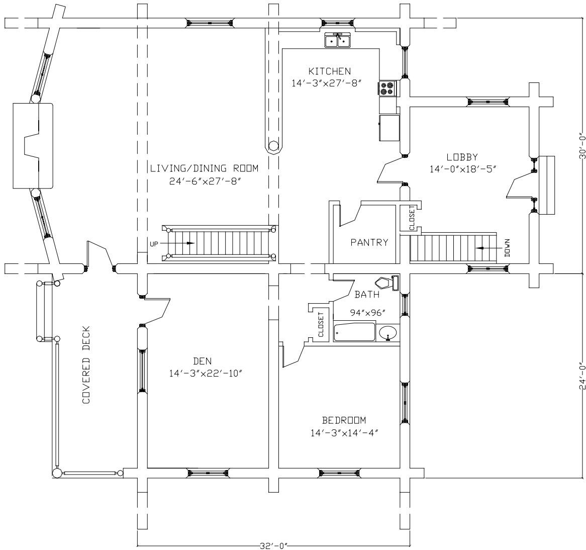
MAIN FLOOR PLAN 2403 SQ.FT.
