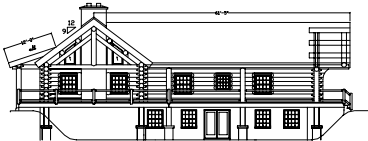
FRONT ELEVATION (PRESUMED GRADE)
