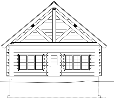
FRONT ELEVATION
