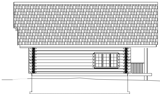
LEFT ELEVATION
