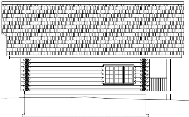
LEFT ELEVATION
